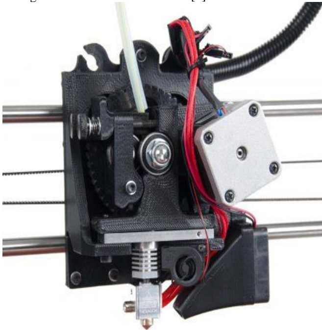
Figure 3(a). Extruder [5]
