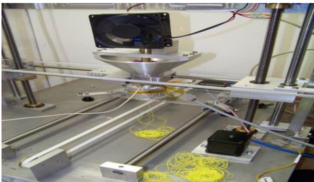
Figure 8. Granulate Extruder [15]
