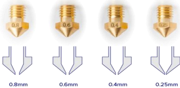
Figure 4. Nozzle [5]
