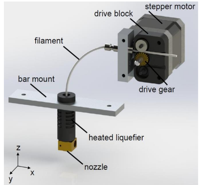
Figure 3(c). Bowden extruder [12]
