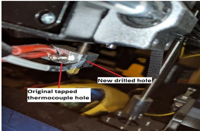
Figure 7. Extruder Heat Block Modification [14]
