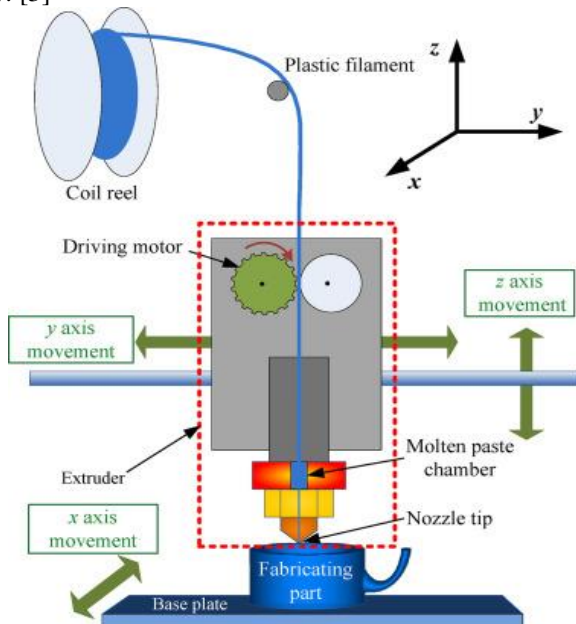
Figure 1. Fused Deposition Modeling (FDM) [11]
