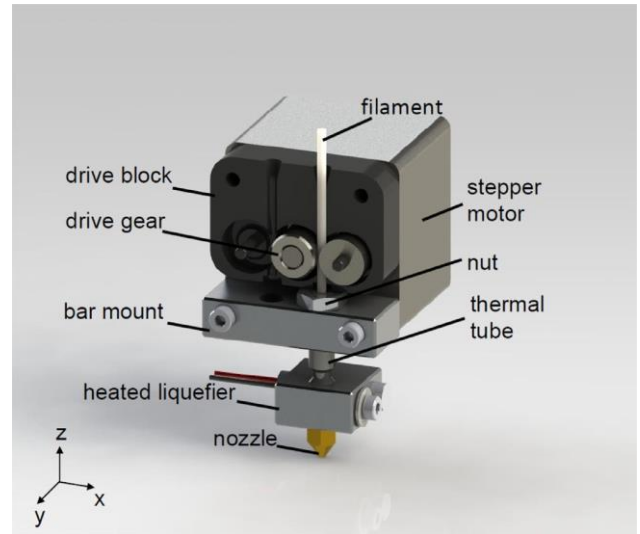
Figure 3(b). Direct extruder [12]
