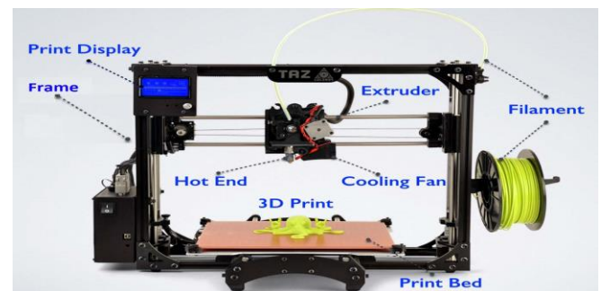
Figure 2. Main components used in FDM 3D printers [5]
